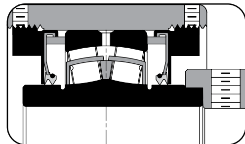
Fig. 15. Double-lip seals.
