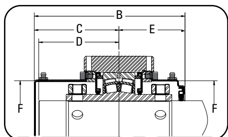
Fig. 29. Single closed-end cover and single open-end cover. (1)
