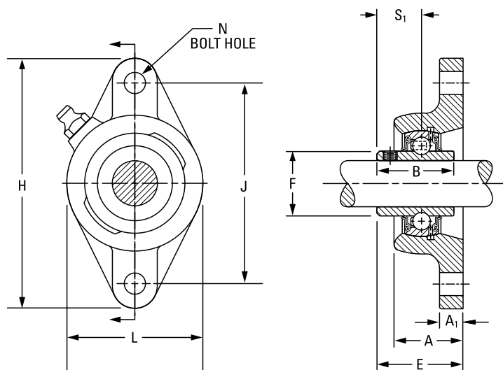
BEARING DATA
