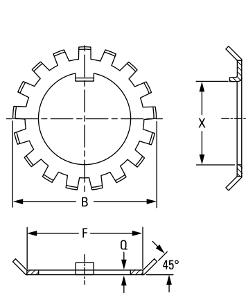
Fig. 50. Lockwashers.
