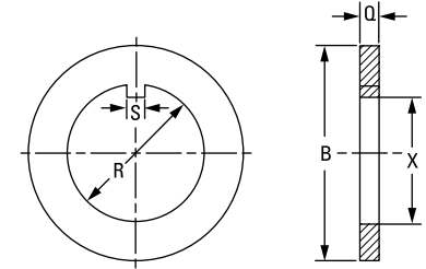
Fig. 51. Tongued washers.
