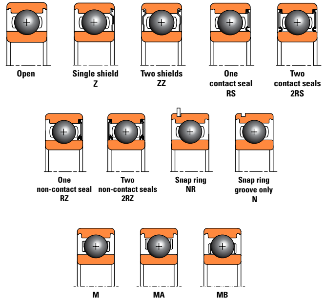
Fig. 1. Deep groove ball bearing configurations.
