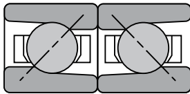
Back-to-Back DB
