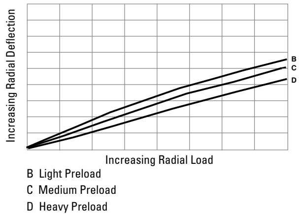
Fig. 19. Effect of contact angle on radial deflection.
