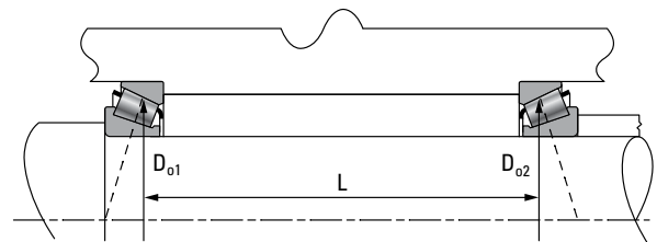
Fig. 94. Resulting distance between bearing geometric centerlines.
