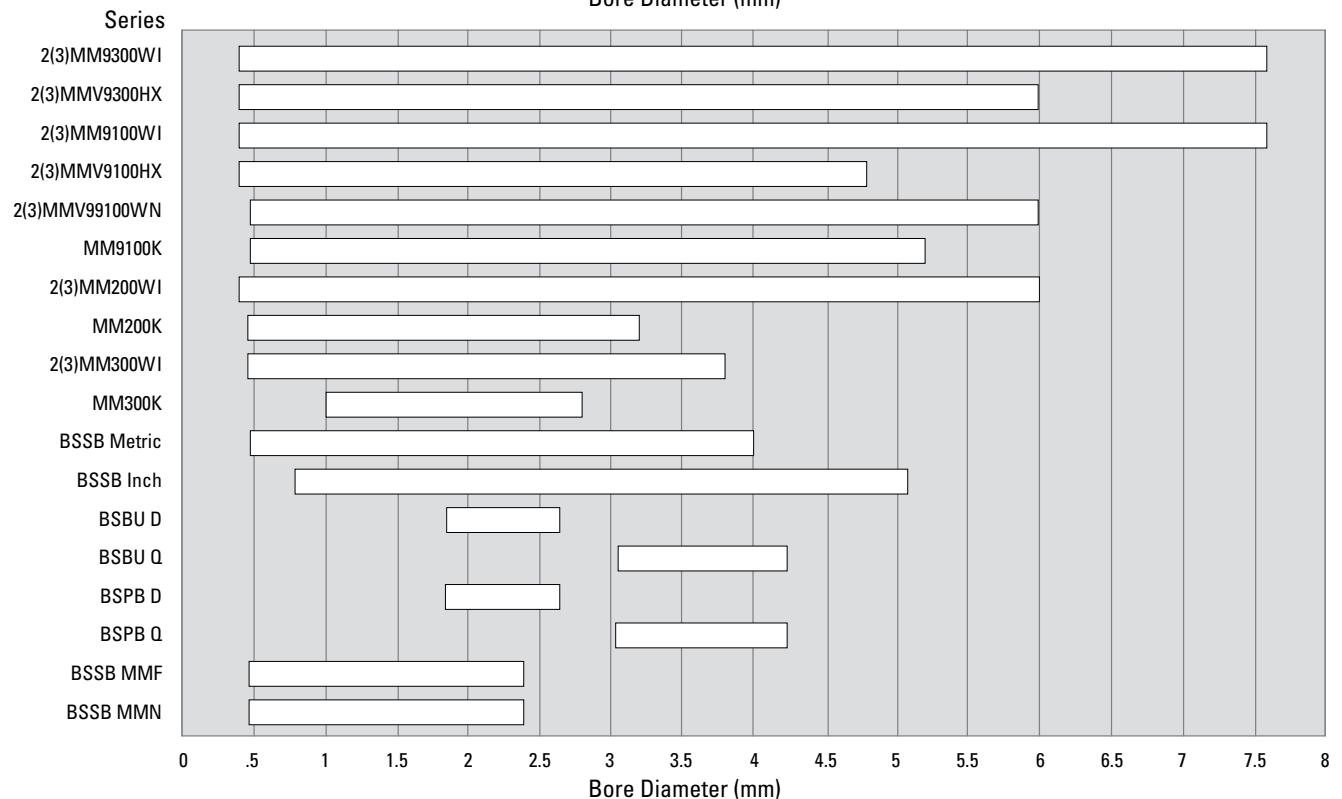
Fig. 136. Bore diameters.
