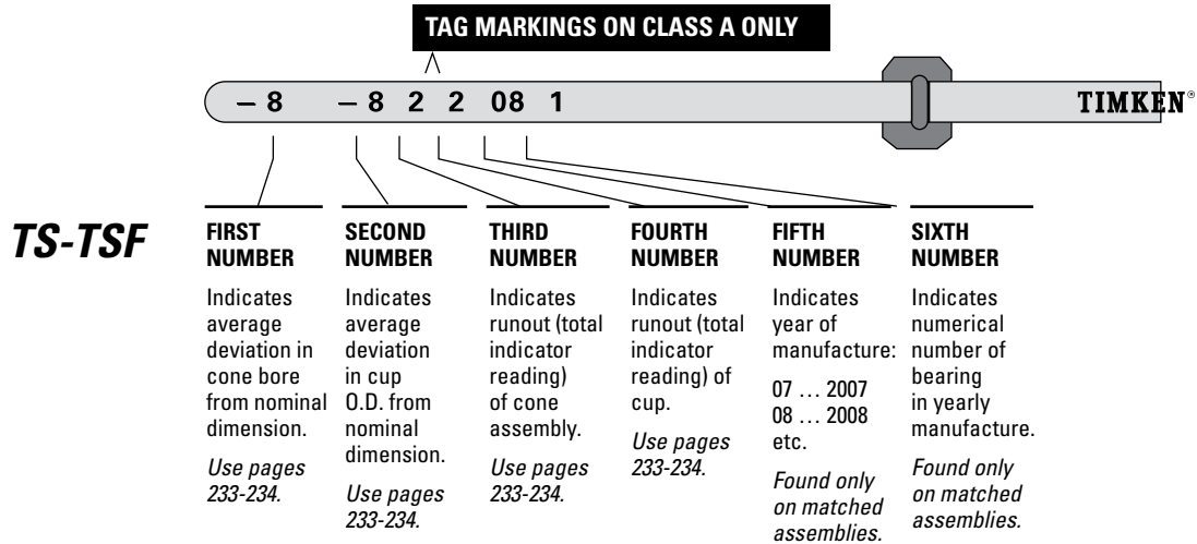
Fig. 101. Metric system precision bearing tag markings.
