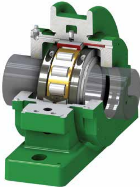
Fig. 4. Retained-type bearings (BR).
