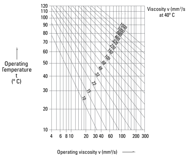
Fig. 13. Operating viscosity.
