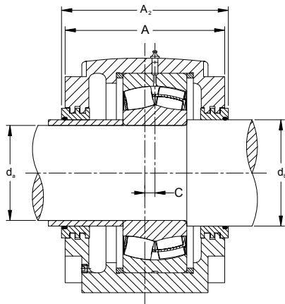
Labyrinth Seal
