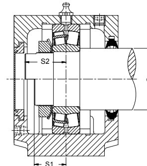
Cylindrical Bore Bearing End Cover / Double-Lip Seal
