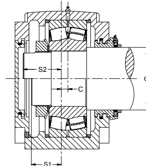
Cylindrical Bore Bearing End Cover / Taconite Seal
