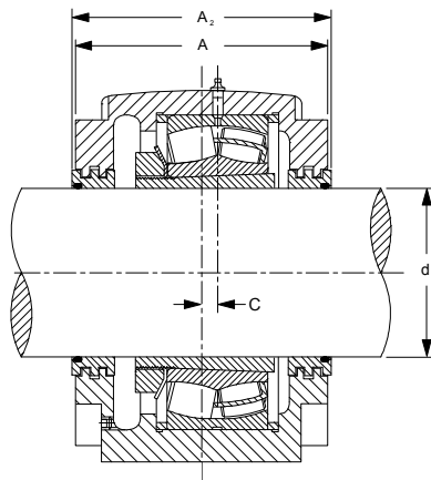
Labyrinth Seal
