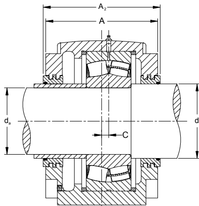
Labyrinth Seal
