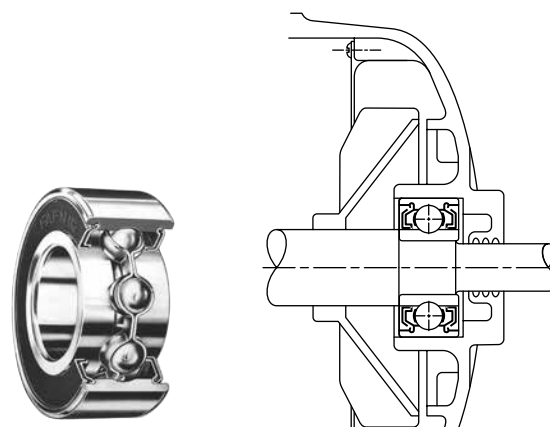
Fig. 168. W-LL-type.
