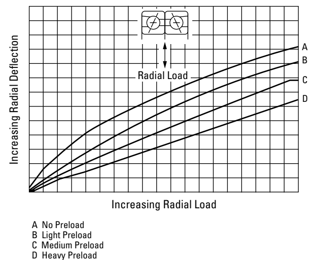
Fig. 140. Effect of most commonly used preloads on radial deflection.
