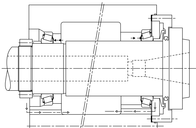
Fig. 118. Simple paired TS mounting with oil inlet at the small end of the rollers.
