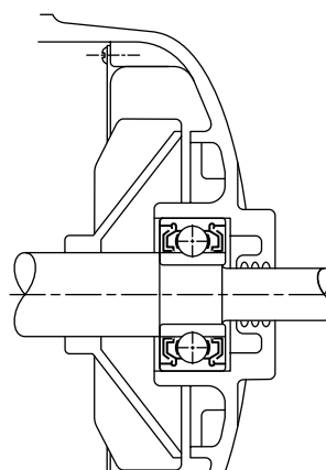
Fig. 169. Typical mounting.
