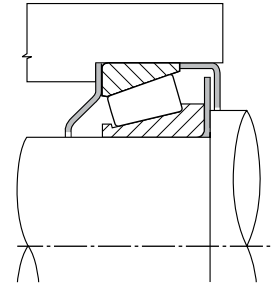
Fig. 152. Metal stampings.
