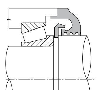
Fig. 154. Machined umbrella flinger combined with annular grooves.
