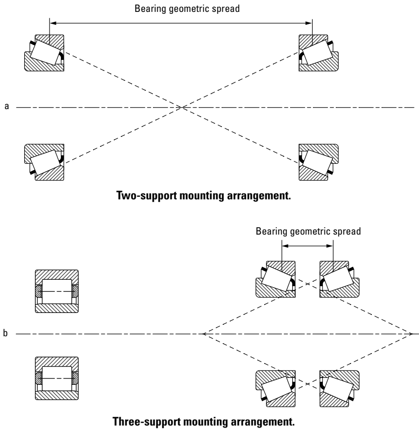
Fig. 137. Mounting arrangements.
