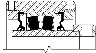
Fig. 11. Eccentric lock.
