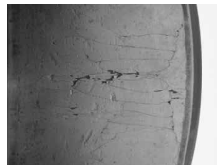
This cylindrical roller bearing inner ring was crushed by an application failure during service.
