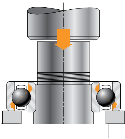
Incorrect removal of a bearing.
