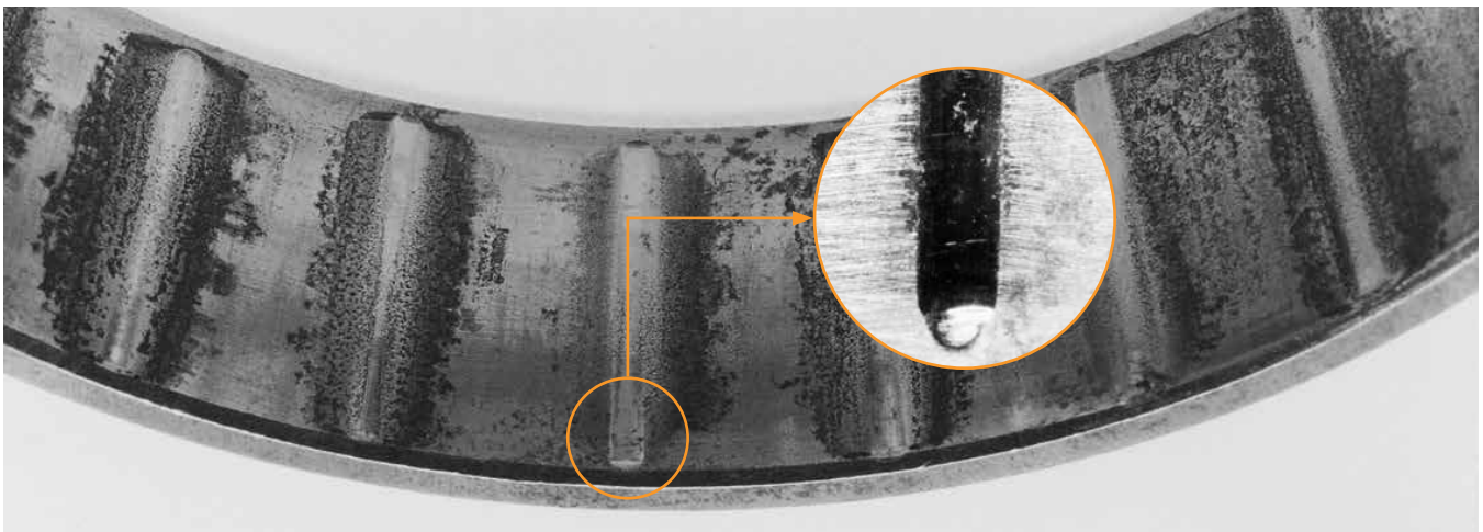
Wear caused by vibration or relative axial movement between the rollers and races is depicted in this tapered roller bearing outer ring.
